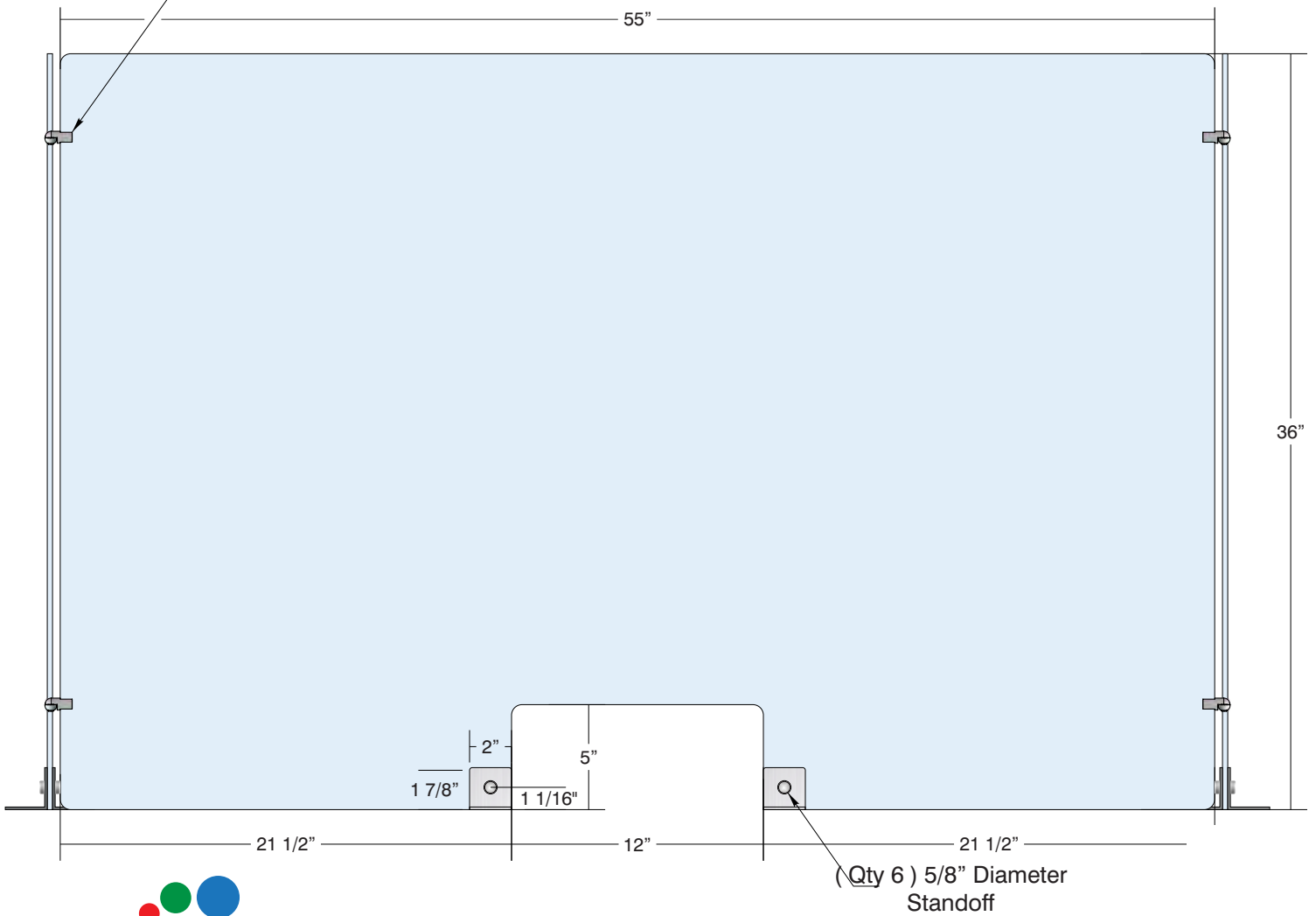
Front View
